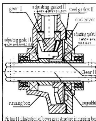
Picture 11 illustration of bevel gear structure in running box
